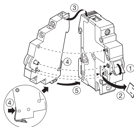
Auxiliary contact
