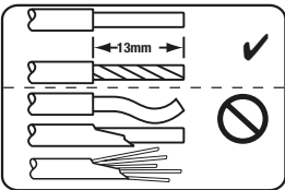
Strip Length
