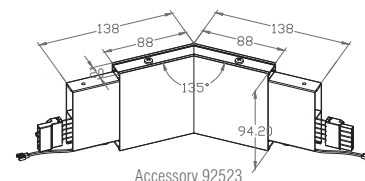
Accessory 92523
