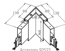
Accessory 92522
