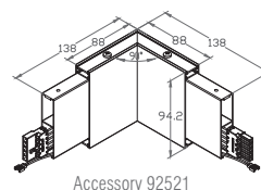
Accessory 92521
